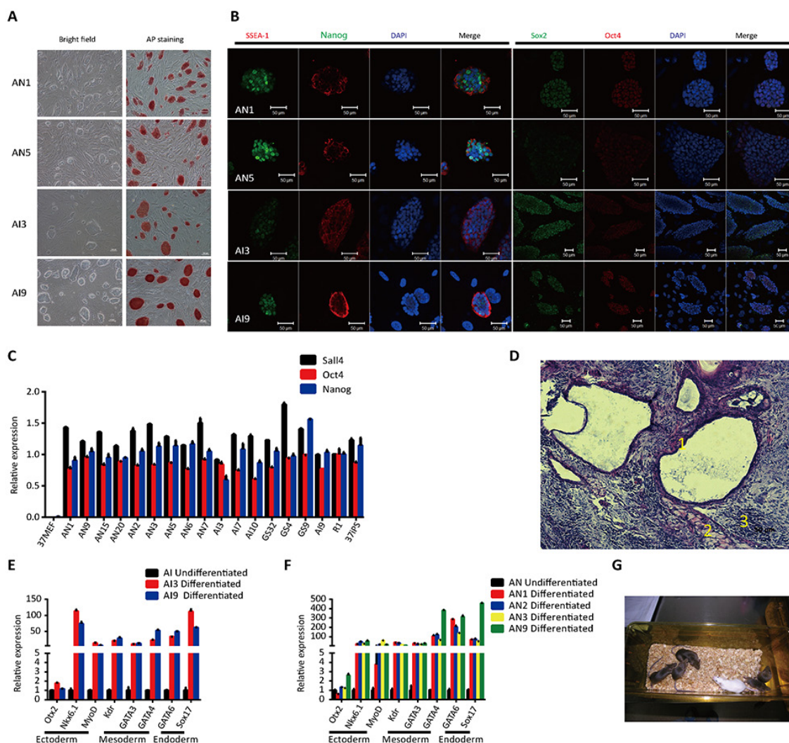
Figure 1: Characteristics of ntESCs and iPSCs from APCs. (A) Morphology and alkaline phosphatase expression of ntESCs and iPSCs. Scale bars, 100 \mu m. (B) Immunofluorescence staining of pluripotent markers SSEA-1 (red), Nanog (green), Sox2 (green), and Oct4 (red) in AN and AI lines. Nuclei were stained with DAPI. Scale bars, 50 \mu m. (C) Quantitative PCR analysis of the pluripotent markers Sall4, Oct4 and Nanog in AN and AI lines. Relative mRNA expression is normalized to GAPDH and is represented relative to expression in fibroblasts (37MEF). The experiments were performed in triplicate (means \pm SD; n=3). The primers used are listed in Supplementary Table 2. (D) H&E staining of teratomas generated from AN1 that formed tissues from all three germ layers. 1: Ectoderm; 2: Mesoderm; 3: Endoderm. Scale bars, 100 \mu m. A detailed description of all of the cell lines is given in Supplementary Table 1. (E and F) Quantitative PCR analysis showing the upregulation of markers for all three germ layers during the in vitro differentiation of AN and AI lines. Relative mRNA expression is normalized to GAPDH and represented relative to expression in undifferentiated AN and AI lines. The experiments were performed in triplicate (mean \pm SD; n=3). The primers used are listed in Supplementary Table 2. (G) Germline transmission of an AN1 tetraploid mouse. Details on all of the cell lines are in Supplementary Table 1.
