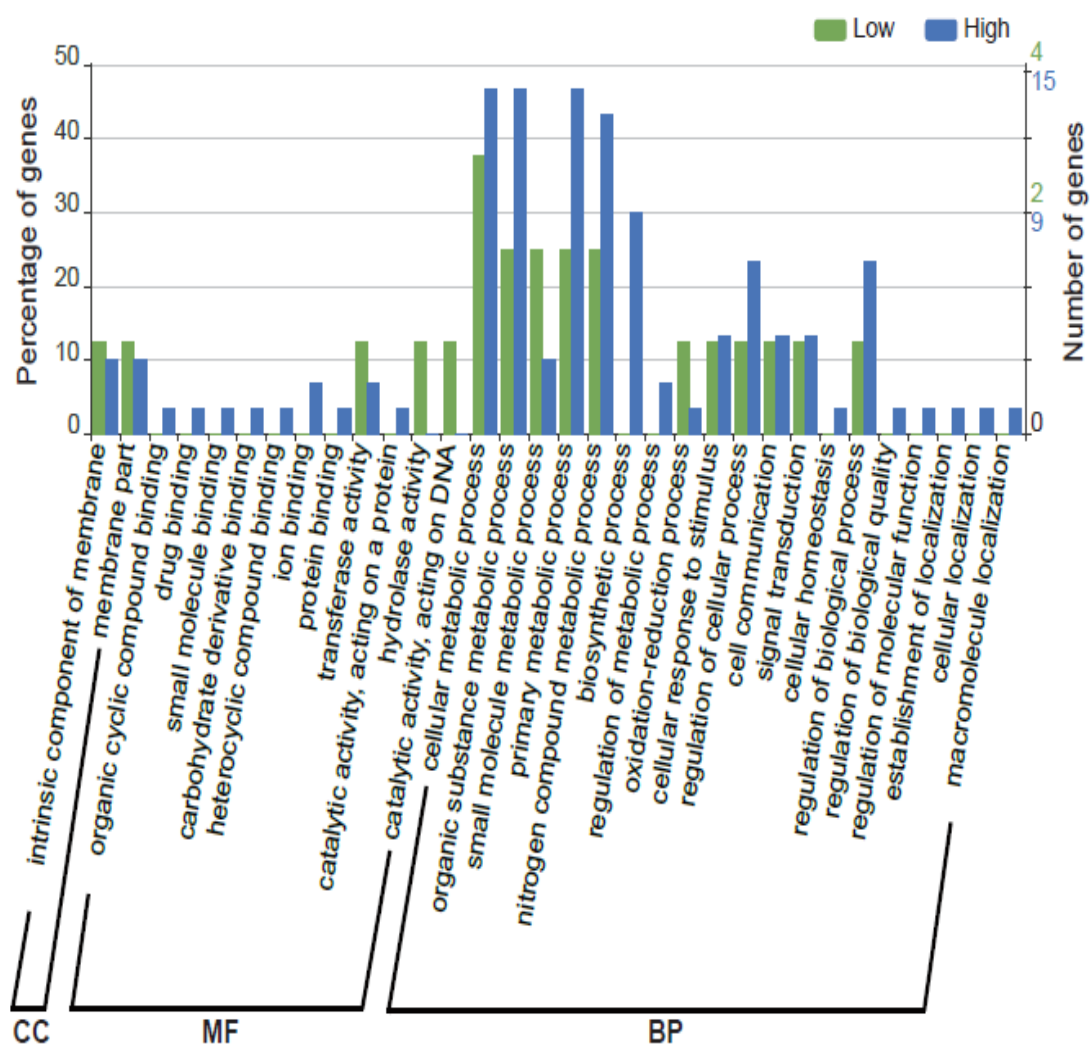
Fig. 2 GO classifications at level 3 for the homologous planthopper proteins shared by all planthopper-virus interactions predicted with the low or high mode. CC, cellular component. MF, molecular function. BP, biological process. In the right vertical axis, green numbers account for the low mode and blue numbers account for the high mode.
